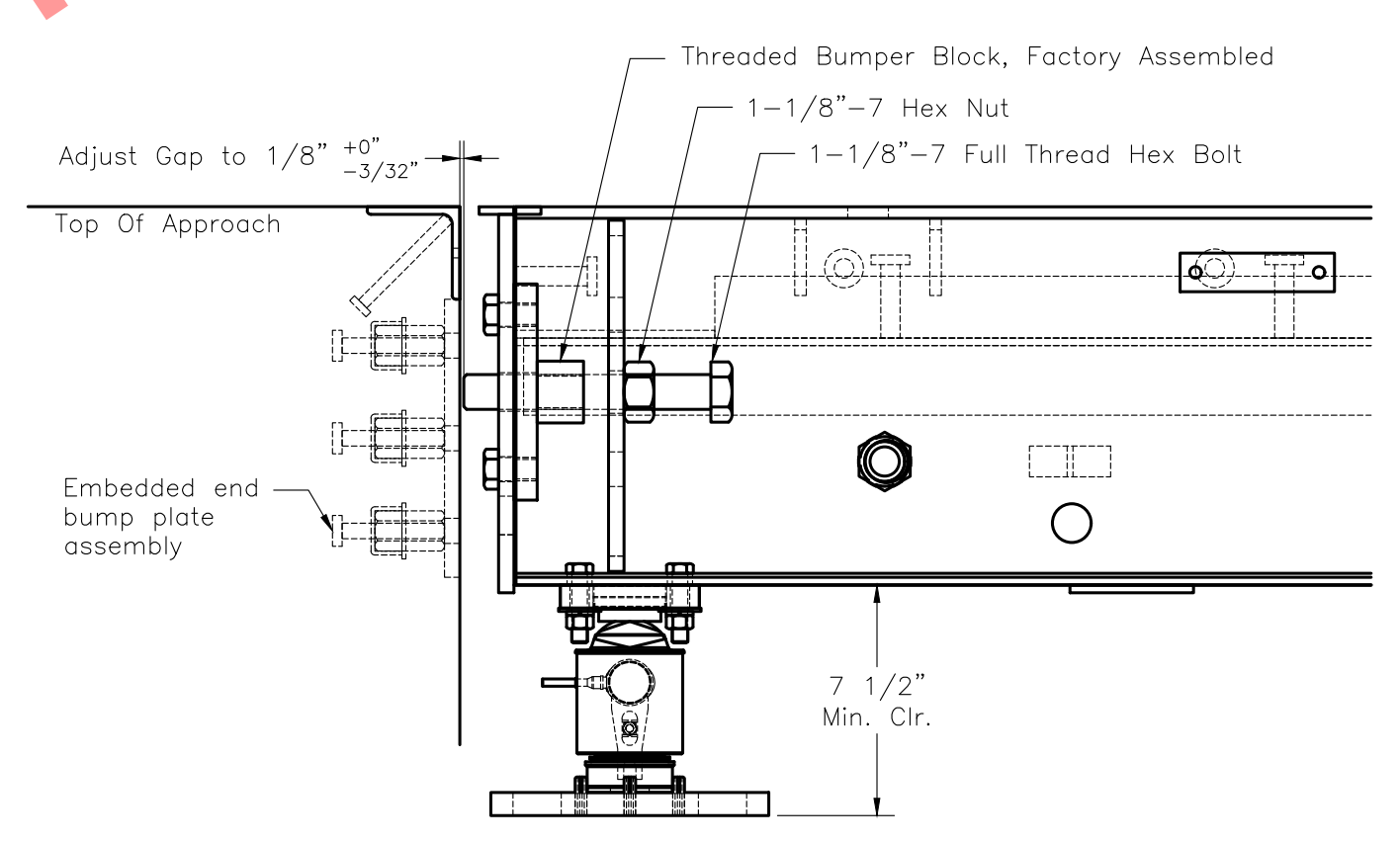
SIDE CHECKING DETAIL Note: Side checking hardware not shown in this view for the sake of clarity
